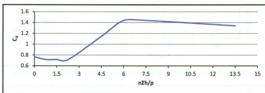
Figure 8: Influence of orifices on the discharge coefficient
