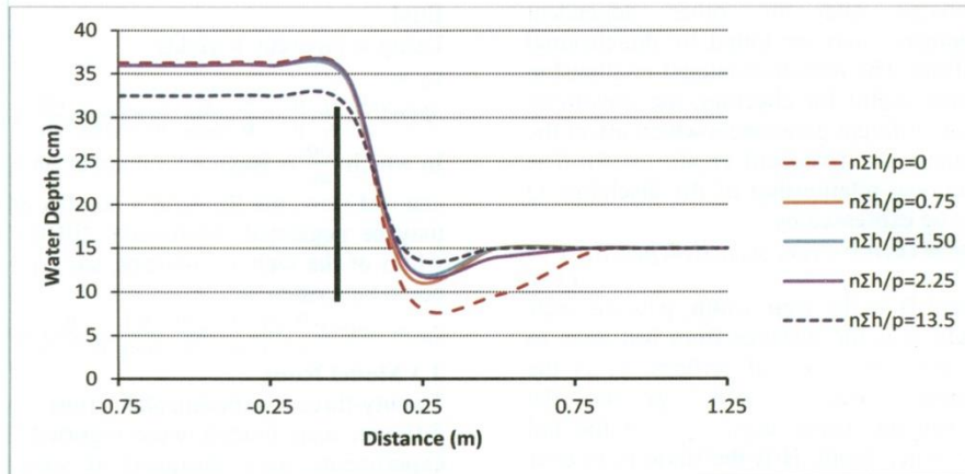
Figure 2: Water surface profile for weir with and without orifices
