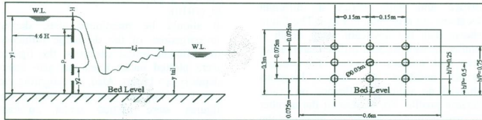
Figure 1: Definition sketch of the used models
