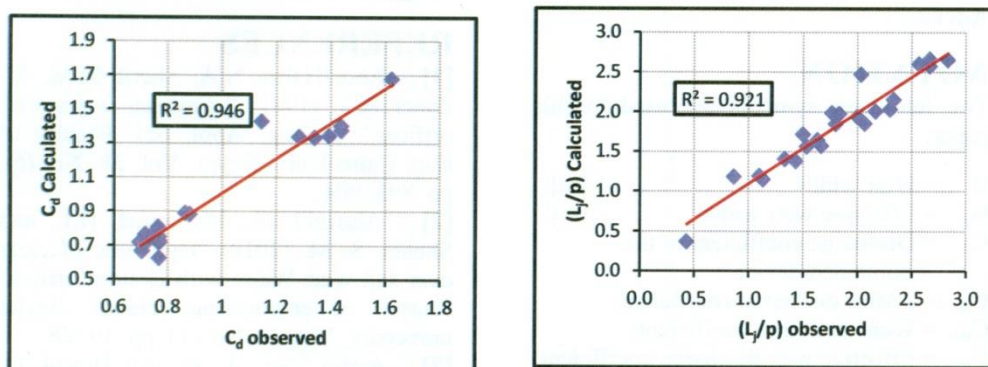
Figure 12: Comparison between observed and calculated values
