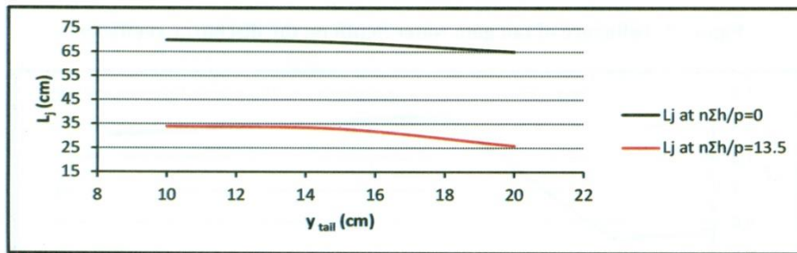
Figure 10: Influence of tail gate water depth on the length of hydraulic jump
