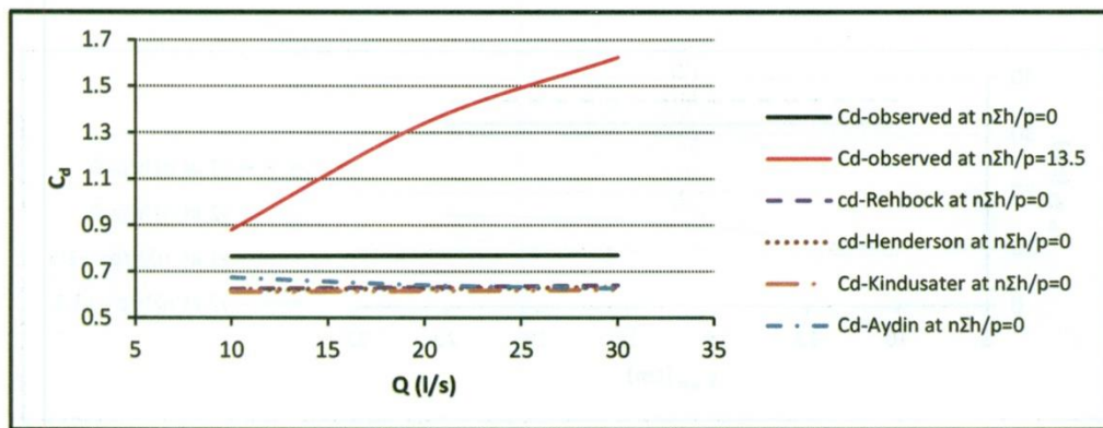
Figure 6: Influence of discharge on the discharge coefficient
