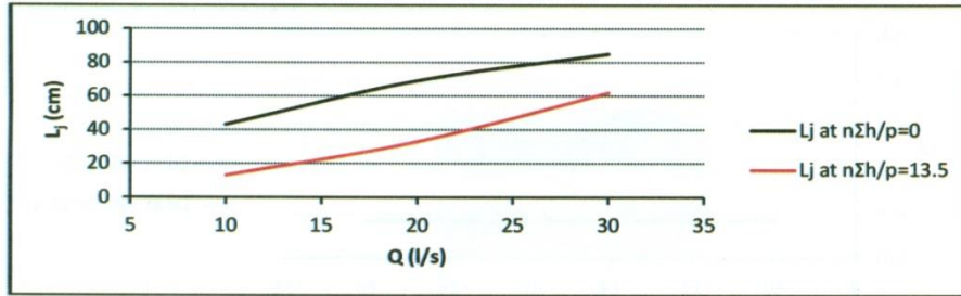
Figure 9: Influence of discharge on the length of hydraulic jump
